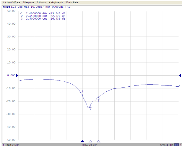
Return Loss
