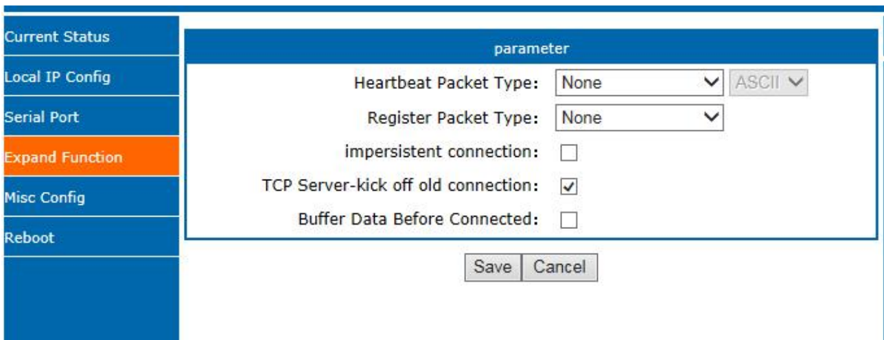
Diagram 4.6.11-1 clear buffer data Configuration
