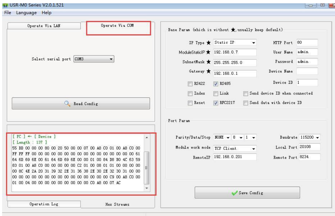
Diagram 5.1.1-6 Port setting
