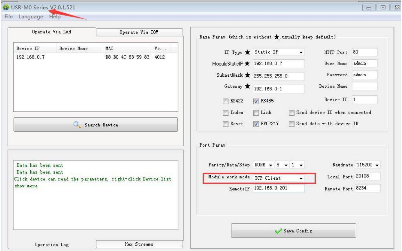
Diagram 4.2.1-1 TCP Client Setting
