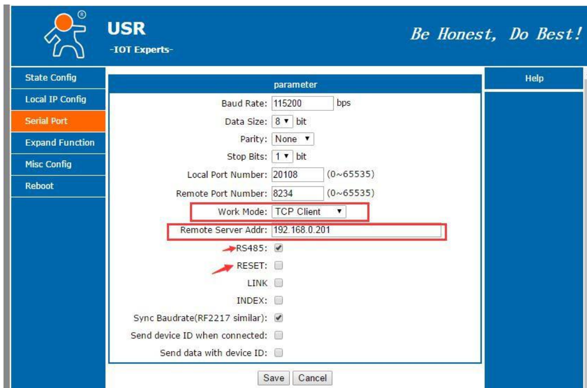
Diagram 5.2.3-1 Serial Port
