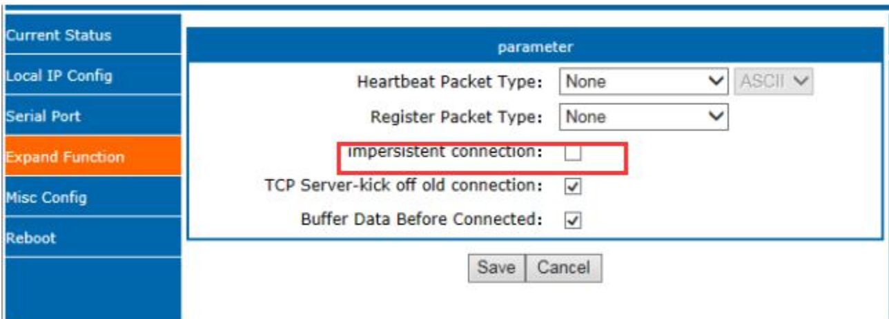
Diagram 4.6.10-1 impersistent connection Configuration
