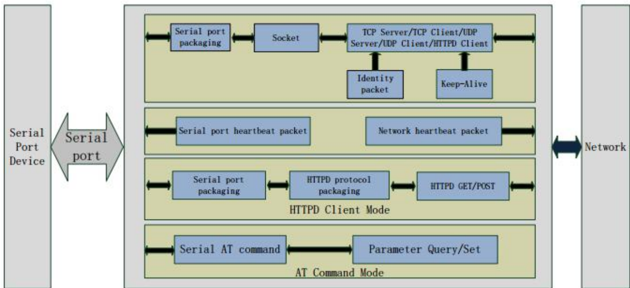
Diagram 4-1 Module Functions
