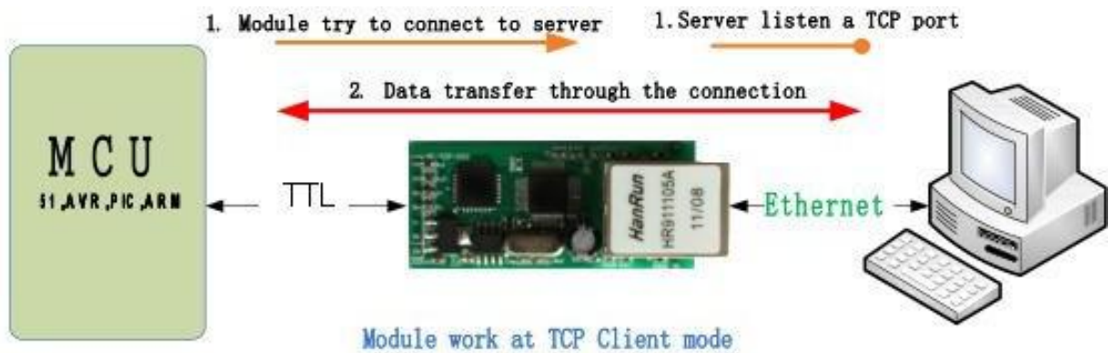
Diagram 4.2.1-2 TCP Client Model
