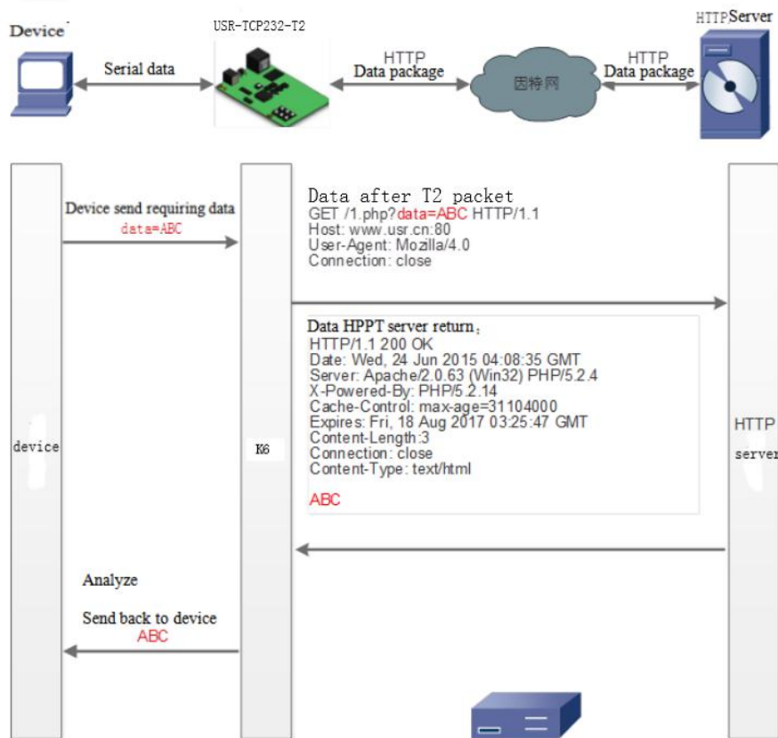
Diagram 4.2.5-1 HTTP client
