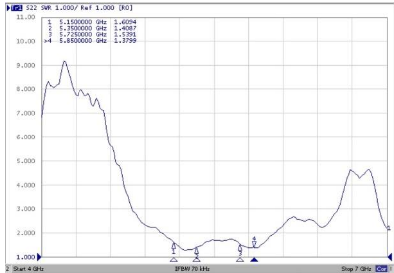
Antenna Port B
